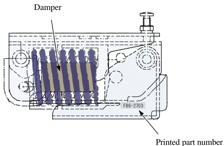
Figure: New type of left hinge unit
